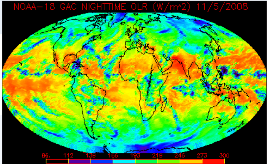
NESDIS Radiation Budget products include daily, monthly, seasonal, and annual mean global maps of outgoing longwave (IR) radiation and absorbed incoming shortwave (solar) radiation. This image, produced on November 5, 2008, shows the Outgoing Longwave Radiative (OLR) flux at the top of the atmosphere. It was derived from NOAA-18 nighttime observations. The NESDIS AVHRR OLR product is used to monitor global climate change and derive the global precipitation index.
